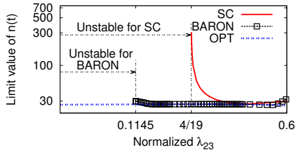
(a) Limit points of the fluid trajectory for variable \hat{\lambda}_{23} .
