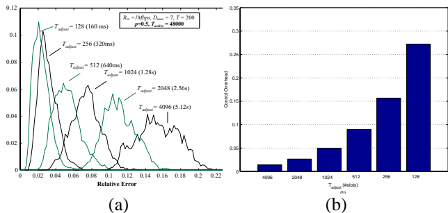
Fig. 11. Effect of frequency of link activations on (a) the average relative error and (b) control overhead.
