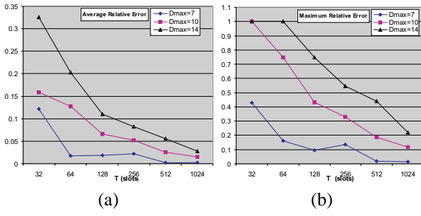
Fig. 7. (a) Average relative error and (b) Maximum relative error for a 100-node static network: p = 1.0 and T_{adjust} = 512 slots. T and D_{max} vary.
