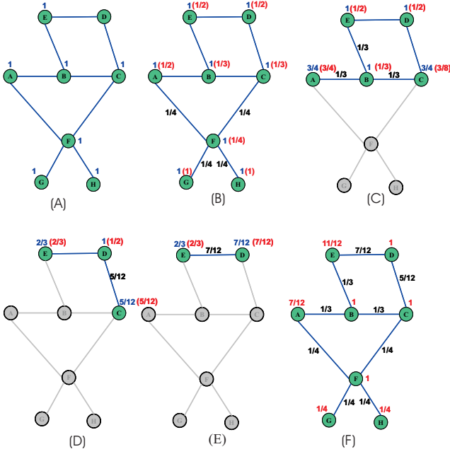
Fig. 2. (a) Initialization: All nodes set their effective capacities to 1 (bipartite topology). (b) Iteration 1: Bottleneck node is F —over all nodes, it provides the minimum fair share of 1/4 to its adjacent links. (c) Iteration 2: Bottleneck node is B (MMF rate is 1/3 ). (d) Iteration 3: Bottleneck node is C (MMF rate is 5/12 ). (e) Iteration 4: Bottleneck node is D , MMF rate is 7/12 . (f) The MMF link rate allocation and corresponding node utilizations.
