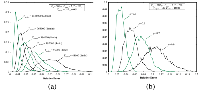
Fig. 10. Effect of (a) rate of topology changes and (b) topology density in the distribution of the average relative error.
