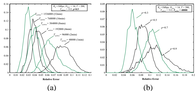
Fig. 12. D_{max} = 14 : Effect of (a) rate of topology changes and (b) topology density in the distribution of the average relative error.
