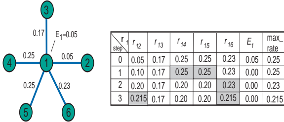
Fig. 3. The FDC algorithm for link (1,2) at node 1 ( C_1 = 1.0, B_{12} = 1.0 ). The shaded entries during each iteration t denote M^{(t)} . The last row is \mathbf{r}'_1 ; the fairness deficit is fd_{1 \rightarrow 2} = 0.215 - 0.05 = 0.165 .
