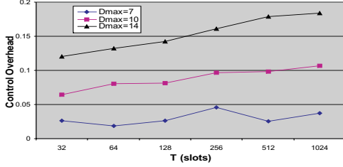
Fig. 8. Control Overhead for a static network of N = 100 , p = 1.0 and T_{adjust} = 512 slots for various choices of T and D_{max} .
