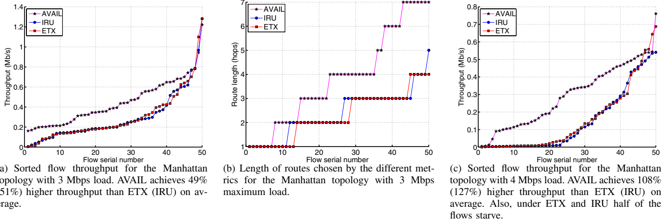
Fig. 16. Manhattan topology
