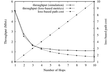
Fig. 9. Throughput over a single path as a function of the number of hops, according to simulation and loss-based metrics
