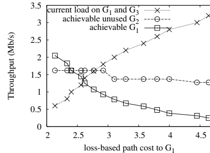
Fig. 14. Load on gateways G_1 and G_3 and achievable throughput on gateways G_1 and G_2 as a function of the corresponding path cost to gateway G_1 , for the example topology of Figure 13
