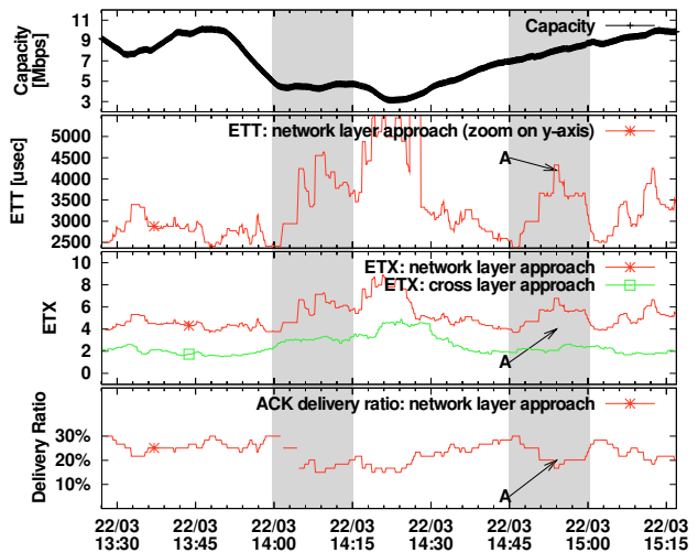
Fig. 6. Dataset A24 in Figure 2. Timeline evolutions of the link capacity, the network layer ETT and some of its components. The gray areas indicates the time intervals discussed in the text.
