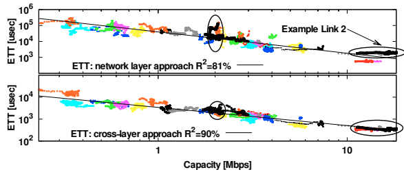
Fig. 5. Scatter plots and fitting lines, in logarithmic scale, of ETT as a function of capacity, across multiple links using auto rate.
