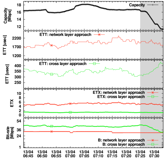
Fig. 9. Timelines of the ETT's components of the "Example link 2" in Figure 5 (auto rate enabled). The gray area indicates the time interval discussed in the text.
