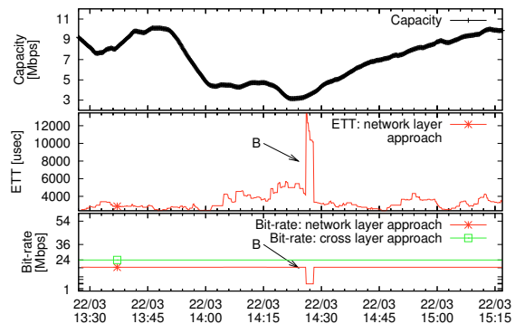
Fig. 7. Dataset A24 in Figure 2. Timeline evolutions of the link capacity, network layer ETT and the link bit-rate estimated by the two approaches.
